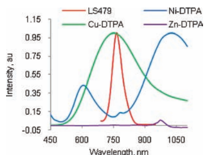
Figure 4. Normalized emission of LS479 ( \lambda_{\text{ex}} = 690 nm) and absorption spectra of \text{Cu}^{2+} -DTPA, and \text{Ni}^{2+} -DTPA and \text{Zn}^{2+} -DTPA (the absorption maximum for the \text{Zn}^{2+} -DTPA complex was <450 nm). Substantial overlap between LS479 and the copper complex suggests that energy transfer is a possible explanation for quenching. The lack of overlap with zinc and nickel should be noted.
