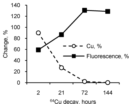
Figure 3. Percent changes in ^{64}\text{Cu}^{2+} concentration as a result of decay (calculated from exponential decay) and in relative fluorescence of Cu-LS479 solution as a function of time. Unquenched LS479 (0.5 \mu\text{M} ) corresponded to a hypothetical zero-time point for fluorescence. Relative fluorescence was measured as an area under the emission curve after addition of ^{64}\text{Cu} solution divided by the area before the addition ( \lambda_{\text{ex}} = 675 nm). An overall increase in fluorescence intensity was seen as a function of time.
